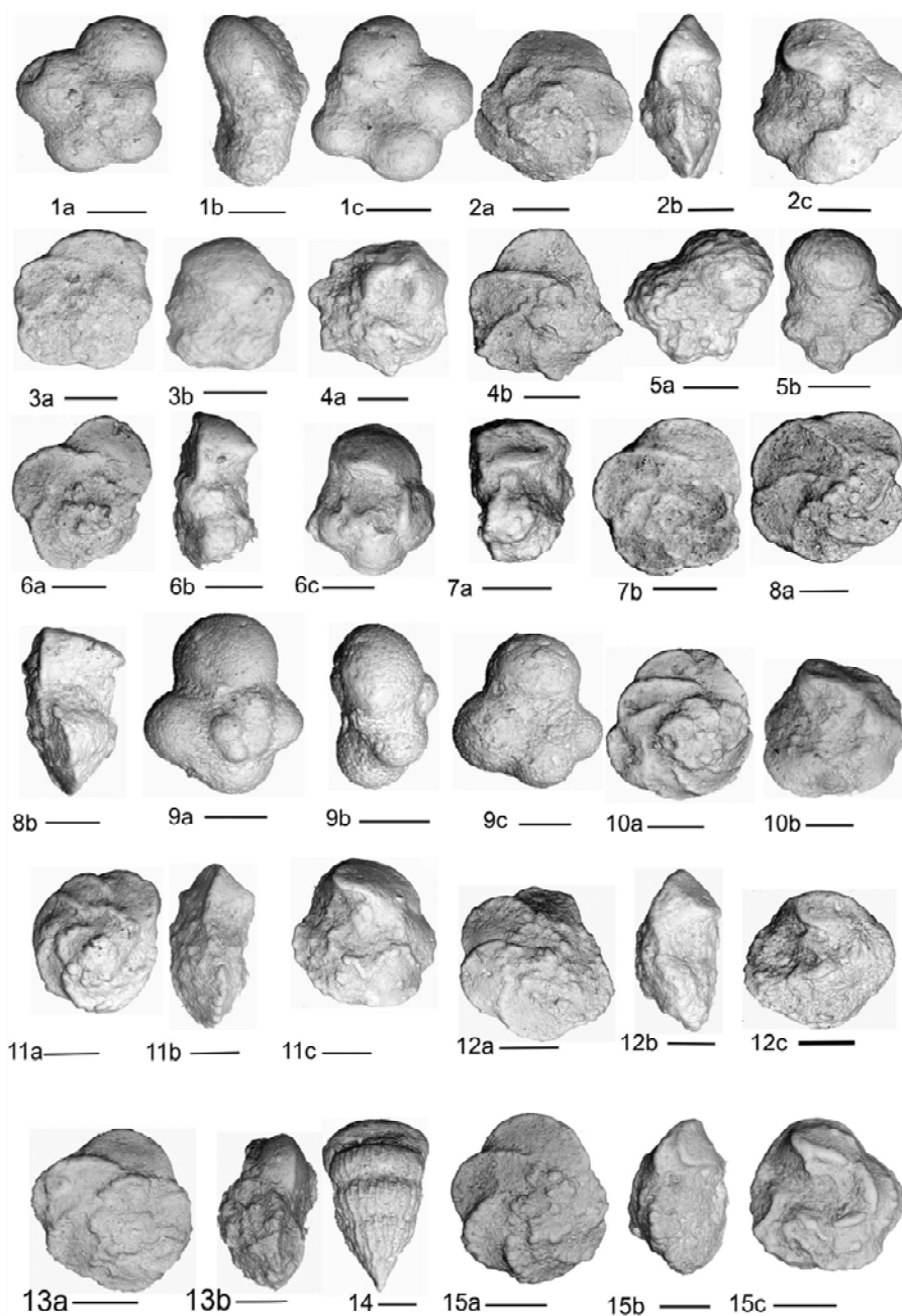
Plate 1. Figure 1a-b: Globotruncanella havanensis (Voorwijk), 1937 (Scale bar: a-b = 50 \mu m; c = 80 \mu m) (placed in zone CF4). Figure 2a-c: Globotruncana esnehensis Nakkady, 1950 (Scale bar = 50 \mu m) (placed in zone CF3). Figure 3a-b: Gansserina gansseri (Bolli), 1951 (Scale bar = 50 \mu m) (placed in zone CF4). Figure 4a-b: Kassabiana pseudocalcarata (Kerdany & Abdelsalam), 1969 (Scale bar: a = 50 \mu m, b = 55 \mu m) (placed in zone CF1). Figure 5a-b: Rugoglobigerina reicheli (Bronnimman), 1952 (Scale bar: a = 45 \mu m, b = 50 \mu m) (placed in zone CF1). Figure 6a-c: Globotruncana aegyptiaca (Nakkady), 1950 (Scale bar = 50 \mu m) (placed in zone CF4). Figure 7a-b: Globotruncanita pettersi (Gandolfi), 1955 (Scale bar = 60 \mu m) (placed in zone CF4). Figure 8a-b: Globotruncanita angulata (Tillev), 1951. (Scale bar; a = 45 \mu m, b = 50 \mu m) (placed in zone CF2). Figure 9a-c: Globotruncanella petaloidea (Gandolfi), 1955 (Scale bar: (a, b = 50 \mu m, c = 60 \mu m) (placed in zone CF4). Figure 10a-b: Globotruncanita stuartiformis (Dalbiez), 1955 (Scale bar = 50 \mu m) (placed in zone CF4). Figure 11a-c: Globotruncanita stuarti (De Lapparent), 1918 (Scale bar = 50 \mu m) (placed in zone CF4). Figure 12a-c: Globotruncana falsostuarti (Sigal), 1952 (Scale bar = 50 \mu m) (placed in zone CF4). Figure 13a-b: Abathomphalus intermedius (Bolli), 1951 (Scale bar: a = 50 \mu m, b = 60 \mu m) (placed in zone CF2). Figure 14: Pseudotextularia elegans (Rzehak), 1895 (Scale bar = 50 \mu m) (placed in zone CF2). Figure 15a-c: Globotruncana arca (Cushman), 1926 (Scale bar = 50 \mu m) (placed in zone CF4).
