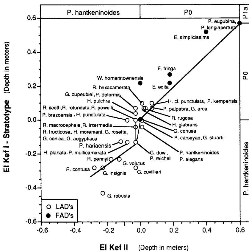
Fig. 6. Graphic correlation of El Kef I and El Kef II sections. Note that El Kef II has either a very condensed topmost Maastrichtian (dotted line) or a short hiatus (solid line).
