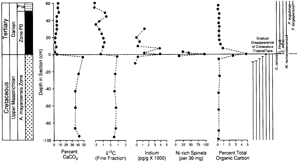
Fig. 2. El Kef I-stratotype showing criteria for placement of the K/T boundary. CaCO 3 , TOC, δ 13 C data from Keller and Lindinger (1989). Iridium and Ni-rich spinel data from Robin et al. (1991). Planktic foraminiferal data from the present study.
