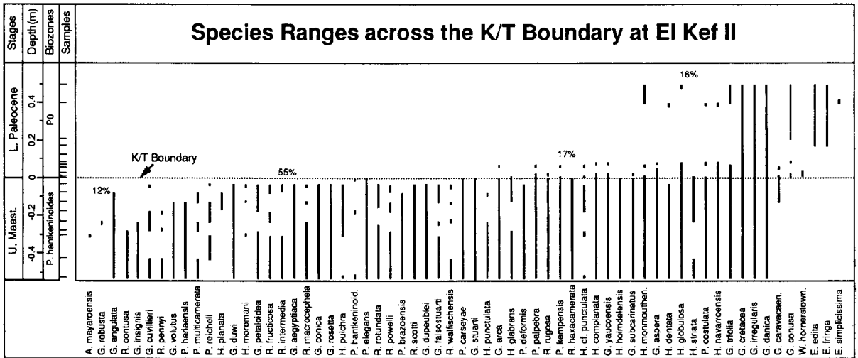
Fig. 5. Biostratigraphic ranges of planktic foraminifera across the K/T boundary at El Kef II.
