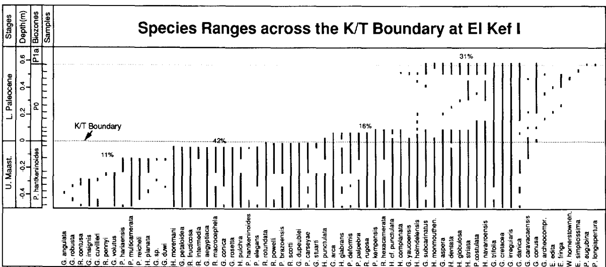
Fig. 4. Biostratigraphic ranges of planktic foraminifera across the K/T boundary at the El Kef I-stratotype.
