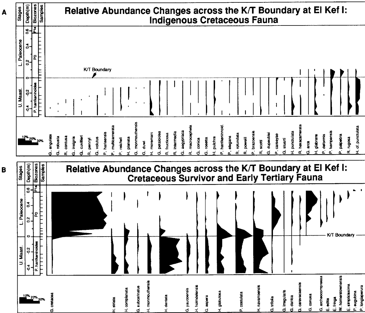
Fig. 9. Relative species abundances of planktic foraminifera in the >63 μm size fraction at El Kef I-stratotype. Note the gradual extinction pattern across the K/T boundary (11A) and the relative abundance changes of Cretaceous survivor taxa (11B).
