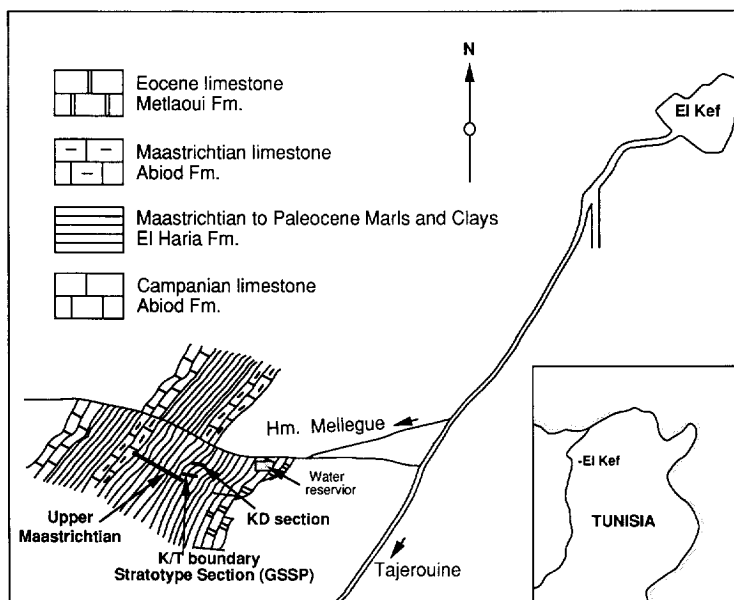
Fig. 1. Location map of the El Kef stratotype section (modified from Donce et al., 1985).
