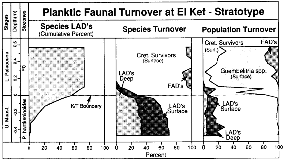
Fig. 11. Selectivity in planktic foraminiferal species extinction and survivorship patterns across the K/T boundary at El Kef I-stratotype. See text for discussion.
