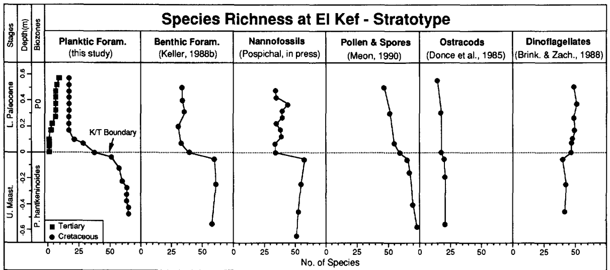
Fig. 12. Species richness patterns in six microfossil groups across the K/T boundary at El Kef I-stratotype. Note that major changes are apparent only in planktic and benthic foraminifera and nannofossils.
