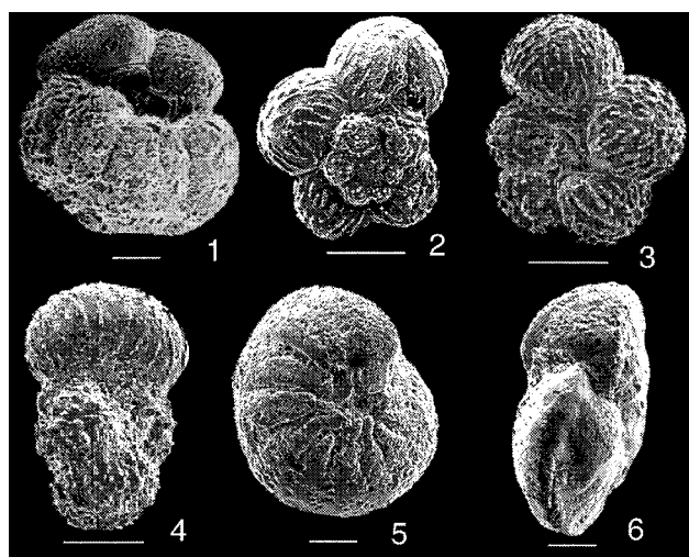
Fig. 5. SEM illustrations of foraminiferal species used for stable isotope analyses and Sr/Ca ratios at El Kef. In all samples scale bar is 100 \mu\text{m} . 1, Rugoglobigerina rotundata (Sample 20–25 cm below the K–T boundary). 2–4, Rugoglobigerina rugosa (sample 10–15 cm below the K–T boundary). 5–6, Anomalinoidea acuta (sample 6 m below the K–T boundary).
