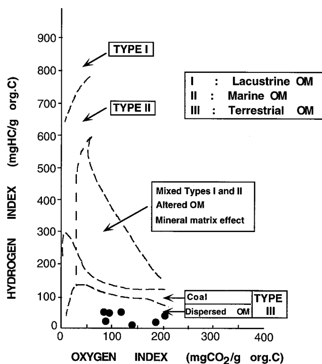
Fig. 9. General HI-OI diagram used for the classification of organic matter type I, II and III. Note that all the high TOC samples analyzed from Tunisian sections are located in the area corresponding to terrestrial OM (Espitalie et al. 1977).
