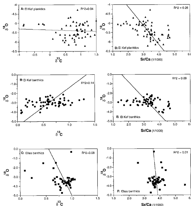
Fig. 6. Plots of \delta^{18}\text{O} v. \delta^{13}\text{C} and \delta^{18}\text{O} v. Sr/Ca ratios at Elles and El Kef. Note that the correlation between these data is weak ( R^2 values between 0.01 and 0.26) and that the cluster of \delta^{18}\text{O} and Sr/Ca values at Elles suggests a high degree of diagenetic alteration in the Elles samples. However, high Sr/Ca ratios correlate with more negative \delta^{18}\text{O} values at El Kef and suggest that diagenetic alteration alone can not explain the more negative \delta^{18}\text{O} values in the El Kef samples. It is likely that diagenetic alteration due to meteoric waters and salinity effects account for the unusually negative \delta^{18}\text{O} values.
