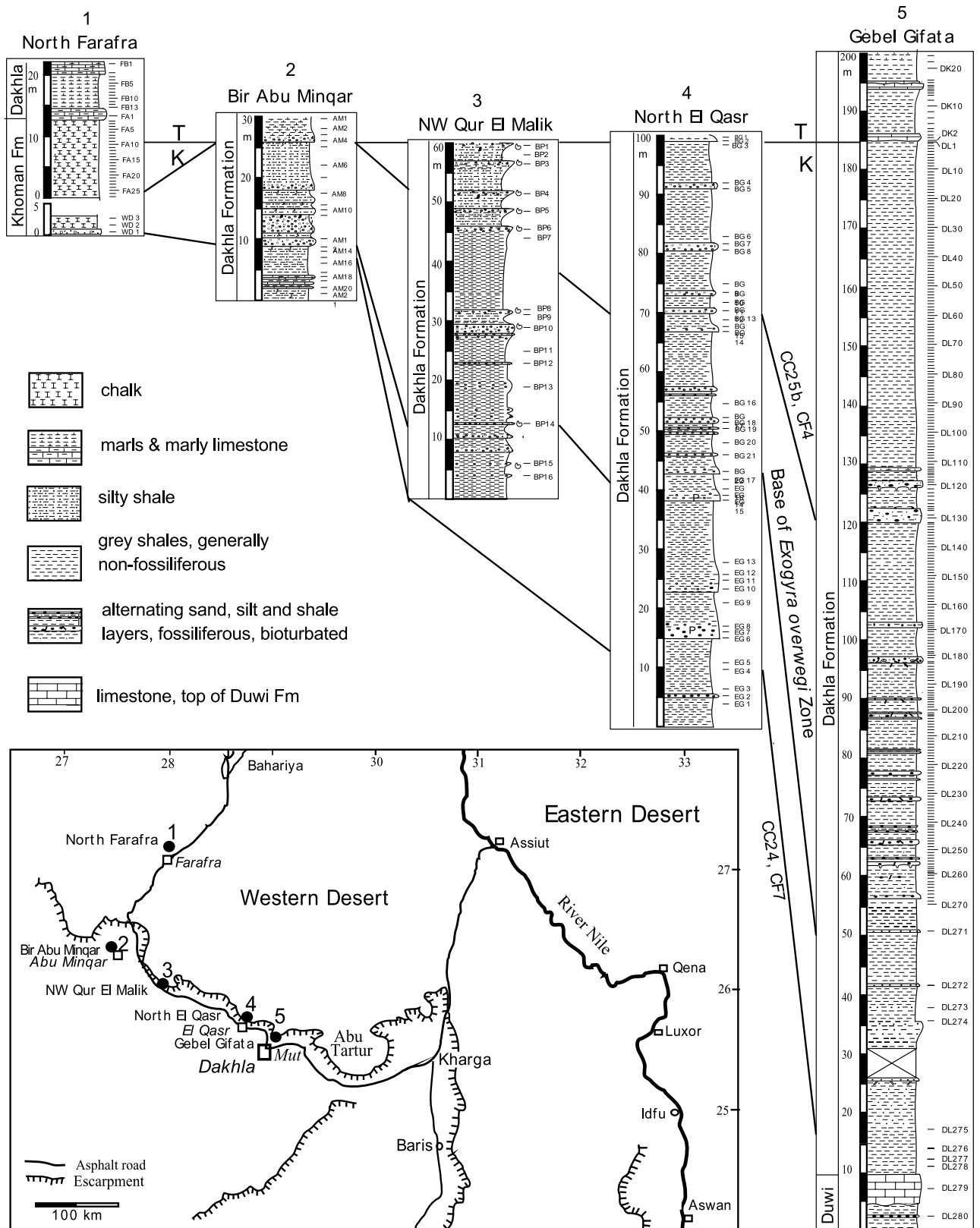
Figure 2. Location map of sections analyzed and their lithological columns correlated based on the K/T boundary disconformity, planktic foraminiferal zones CF4 and CF7, calcareous nannofossil zones CC25b and CC24, and the base of the Exogyra overwegi Zone. Note that in Northwest Qur El Malik no microfossils were recovered, although macrofossils are present.
