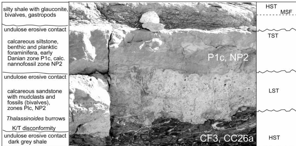
Figure 17. Sequence stratigraphy and sea-level changes across the Cretaceous/Tertiary boundary disconformity at Gebel Gifata. The disconformity juxtaposes the late Maastrichtian planktic foraminiferal zone CF3 and calcareous nannofossil zone CC26a with the early Danian Bir Abu Minqar horizon of planktic foraminiferal zone P1c and calcareous nannofossil zone NP2 age. The undulating erosional surfaces between the dark shale and calcareous sandstone layers at the top and bottom, and within the calcareous sandstone layer mark changes in sea levels.
