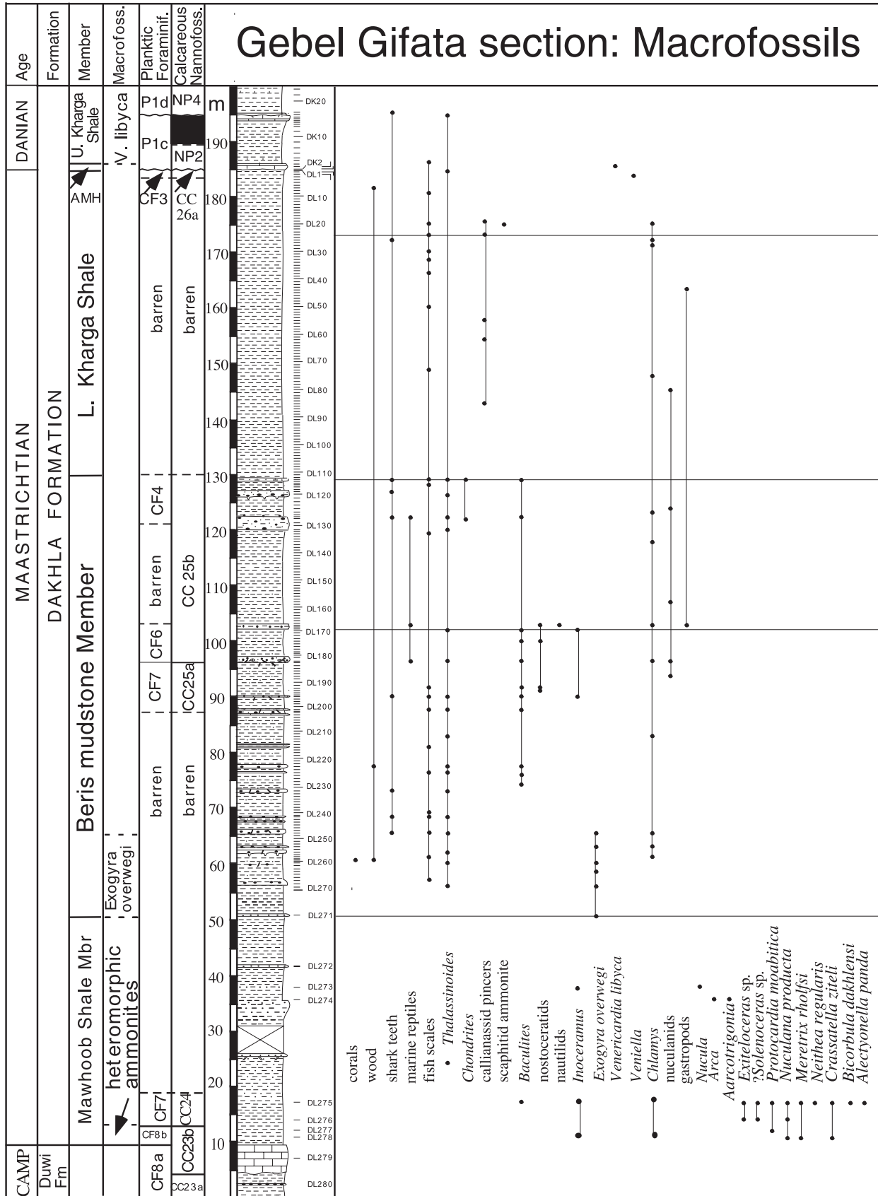
Figure 3. Lithological column, sample intervals, integrated microfossil and macrofossil biostratigraphies, and macrofossil ranges at the Gebel Gifata section for the Late Campanian–Early Paleocene.
