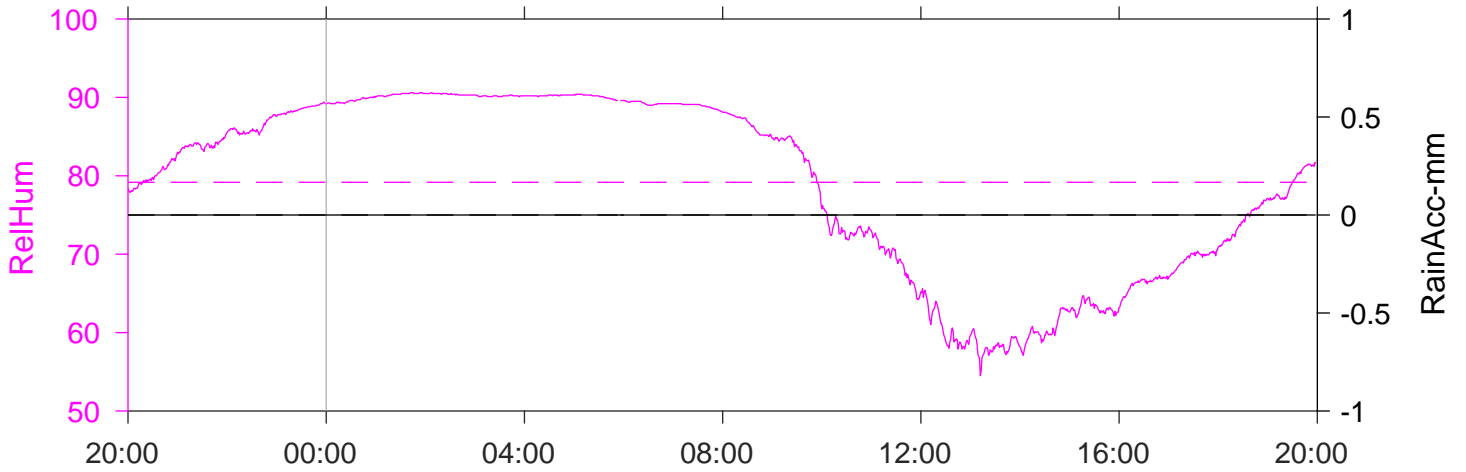
RelHum / RainAcc-mm 27-Sep-2020 (UTC day 271)
