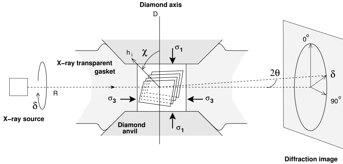
Fig. S2: Schematic of the experiment. The polycrystalline sample is confined under non-hydrostatic stress conditions between the two diamond anvils. \sigma_1 is the axial stress imposed by the diamonds and \sigma_3 the radial stress imposed by the gasket. A monochromatic x-ray beam is sent through the gasket and the data collected on an imaging plate orthogonal to the incoming beam. The position of the diffraction lines and intensity of diffraction are analyzed as a function of the azimuthal angle \delta from which we calculate the angle \chi between the normal to the diffracting plane h_i and the compression direction.
