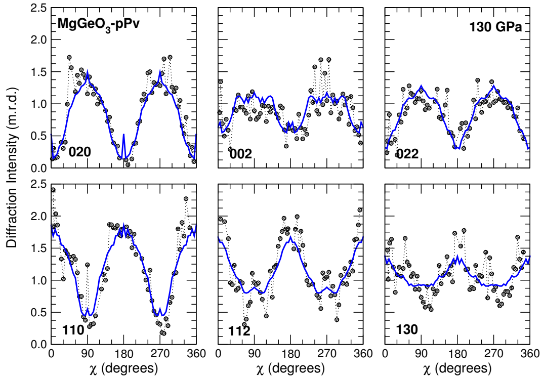
Fig. S3: Measured diffraction intensities using the single peak fitting techniques (closed circles) and those recalculated from the orientation distribution function (solid blue lines) as a function of the pole distance \chi for the peaks 020, 002, 022, 110, 112, and 130 of \text{MgGeO}_3\text{-pPv} at 130 GPa. Experimental intensities have been scaled to match those recalculated from the ODF, expressed in m.r.d.
