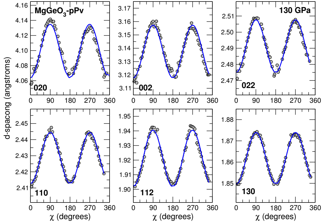
Fig. S4: Measured d-spacing using the single peak fitting techniques (closed circles) and models used for lattice strain analysis (solid blue lines) as a function of the pole distance \chi for the peaks 020, 002, 022, 110, 112, and 130 of MgGeO 3 -pPv at 130 GPa.
