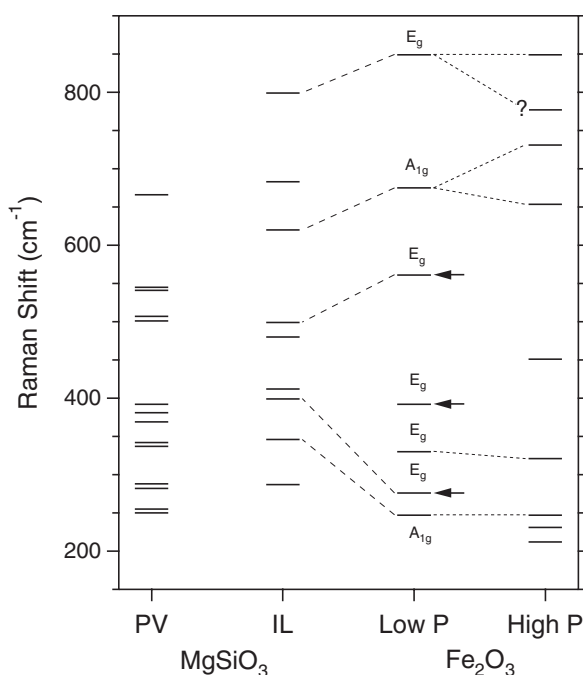
FIGURE 8. Raman modes before and after the phase transformation for Fe 2 O 3 at 55 GPa. Modes for MgSiO 3 ilmenite and perovskite phases are shown for comparison. Group theoretical correlation between MgSiO 3 ilmenite and Fe 2 O 3 corundum phases are shown by dashed lines. Peak splitting and continuation through phase transformation in Fe 2 O 3 system is denoted by short dashed lines. The modes that disappear after the phase transformation are highlighted by arrows. “?” denotes a new mode observed only during decompression.
