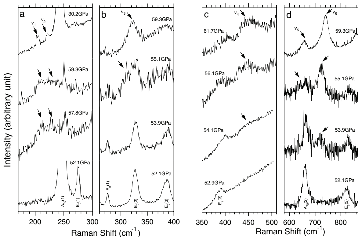
FIGURE 7. Raman spectra of \text{Fe}_2\text{O}_3 showing evidence for high-pressure phase transformation for (a) 170–300 \text{cm}^{-1} , (b) 260–400 \text{cm}^{-1} , (c) 350–510 \text{cm}^{-1} , and (d) 590–835 \text{cm}^{-1} . The new peaks are highlighted by arrows. Assignments for the low-pressure phase are given. In (a) 30.2 GPa spectrum was obtained during decompression.
