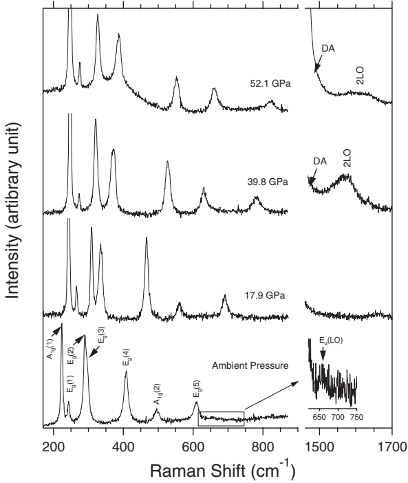
FIGURE 2. Representative Raman spectra of hematite to 52.1 GPa. The spectra are normalized to the intensity of the E_g(2) mode. Raman signal from the diamonds is indicated with “DA.” Peak assignment is shown for each phonon mode. The 620–750 \text{cm}^{-1} range is shown in the inset to illustrate the observation of Raman-inactive and IR-active E_u(\text{LO}) mode.
