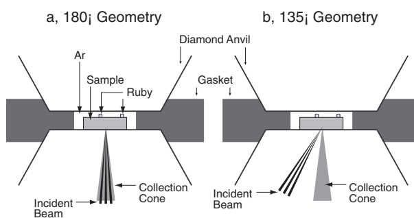
FIGURE 1. Experimental setup for (a) 180^\circ and (b) 135^\circ scattering geometries.
