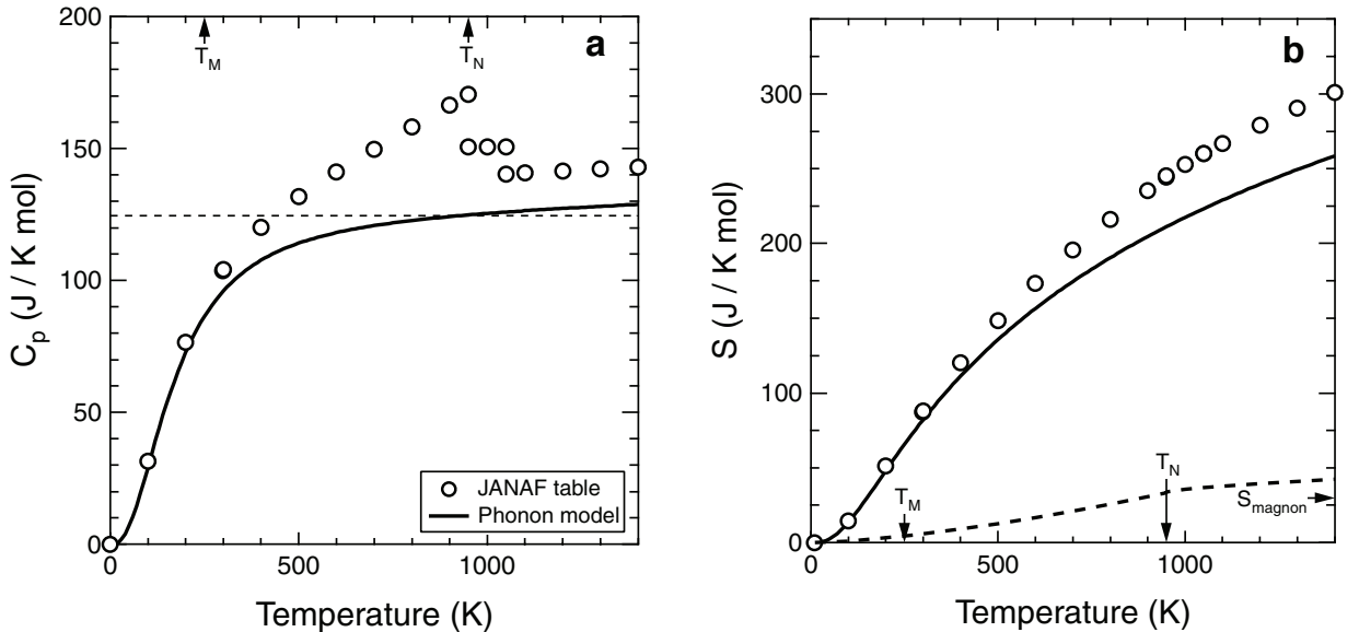
FIGURE 6. (a) Isobaric heat capacity, C_p , and (b) entropy, S , from calorimetry (open circles; Chase 1998) and from Kieffer's model using phonons measured in this study (solid line). Morin temperature ( T_M ), Néel temperature ( T_N ), and empirical calculation of magnon entropy contribution, S_{\text{magnon}} , are shown with arrows. The Dulong-Petit limit is shown by a dashed line in (a). The difference between the calorimetrically measured and calculated entropy is shown by a dashed line in (b) to compare with the empirical calculation for the magnon contribution.
