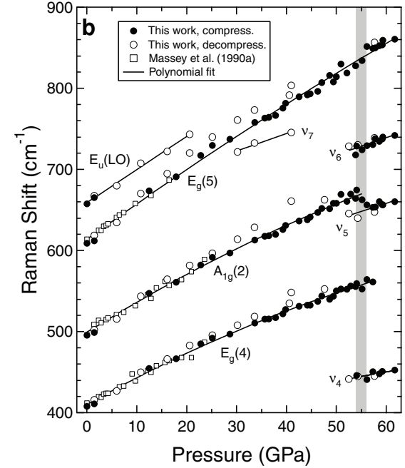
FIGURE 3. Pressure-induced frequency shifts of phonon modes. Solid circles indicates data measured during compression and open circles are data measured during decompression. The measurements of Massey et al. (1990a) are shown by open squares. The solid lines are polynomial fits to the data. Polynomial fits are required due to the significant nonlinearity of all modes. New modes for the high-pressure phase are assigned as \nu_i ( i = 1-7 ) in order of lowest wave number. The pressure range where we observed changes in the Raman spectrum is indicated by gray shading.
