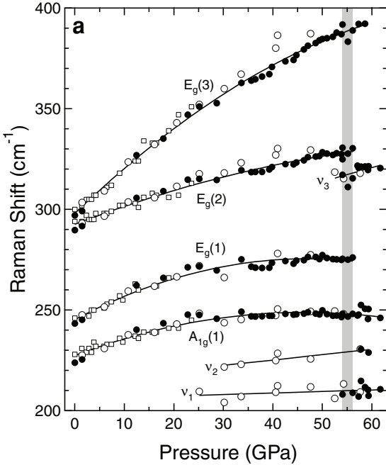
FIGURE 3. Pressure-induced frequency shifts of phonon modes. Solid circles indicates data measured during compression and open circles are data measured during decompression. The measurements of Massey et al. (1990a) are shown by open squares. The solid lines are polynomial fits to the data. Polynomial fits are required due to the significant nonlinearity of all modes. New modes for the high-pressure phase are assigned as \nu_i ( i = 1-7 ) in order of lowest wave number. The pressure range where we observed changes in the Raman spectrum is indicated by gray shading.
