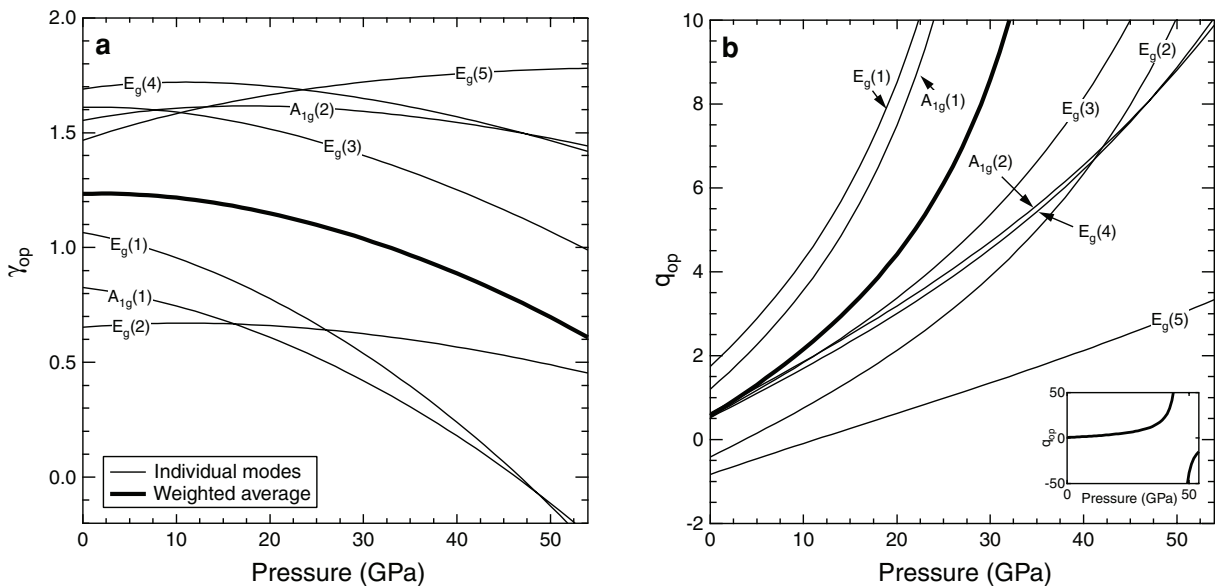
FIGURE 5. (a) Grüneisen parameter, \gamma , and (b) its logarithmic volume derivative, q , for each phonon mode and their weighted average as a function of pressure. The inset in (b) illustrates the singularity of q for the average.
