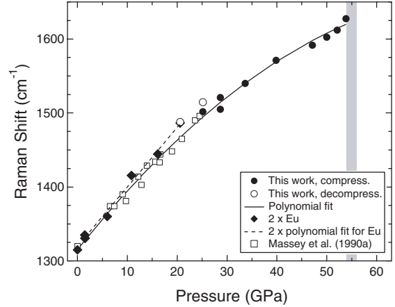
FIGURE 4. Pressure induced shift of 1320 cm -1 mode. Notation is the same as in Figure 3. The solid diamonds and dashed line shows twice the frequency of the E_u(\text{LO}) mode.
