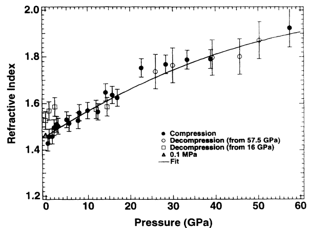
FIG. 5. Pressure dependence of refractive index in SiO 2 glass on compression and decompression. The triangle shows the one-bar refractive index.
