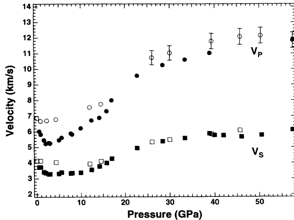
FIG. 3. Sound velocities in SiO 2 glass as a function of pressure. Solid symbols, compression; open symbols, decompression.
