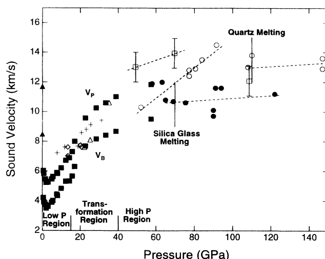
FIG. 10. Sound velocities in silica glass and quartz under shock compression compared with compressional and bulk velocities under static compression (solid squares). The vertical lines at 70 and 110 GPa show the approximate location of melt boundaries under shock compression for silica glass and quartz, respectively. Hugoniot data for silica glass are shown by the solid circles (Ref. 14) and diamonds (Ref. 56), other symbols are for quartz starting material (pluses) (Ref. 55); open triangles (Ref. 54); open squares (Ref. 57); open circles (Ref. 14). Dashed lines serve to connect different data sets at high pressure. The solid triangles show the ambient pressure (0.1 MPa) compressional and bulk sound velocities for stishovite (Ref. 52).
