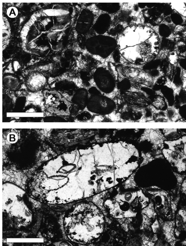
Fig. 4. (A and B) Microphotographs of thin sections showing characteristics of the early Danian (Zone Pla) spherule-rich deposit at Coxquihui. Note the abundance of rounded marl and carbonate clasts and shell fragments that suggest reworking. Terrigenous detritus is rare. Scale bar: 0.5 mm.
