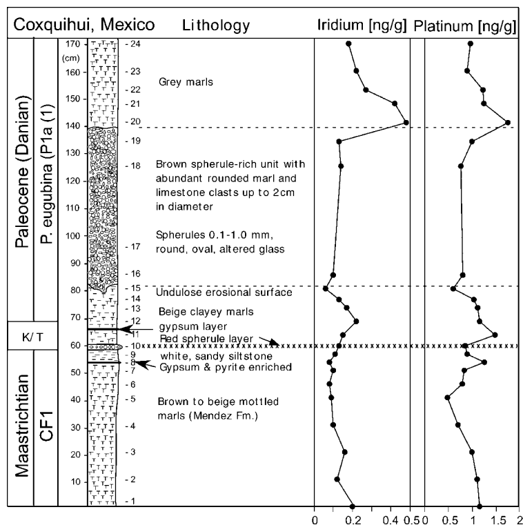
Fig. 3. Lithology, and distribution of iridium and platinum across the K/T transition at Coxquihui, State of Vera Cruz, Mexico.
