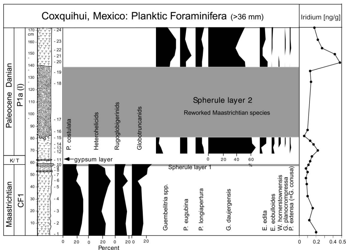
Fig. 6. Relative abundances of planktic foraminifera and Ir distribution across the K/T transition at Coxquihui. Note the high abundance of very small early Danian P. eugubina Zone Pla(l) assemblages below spherule layer 2, and the Ir anomaly in the marls above this spherule layer.
