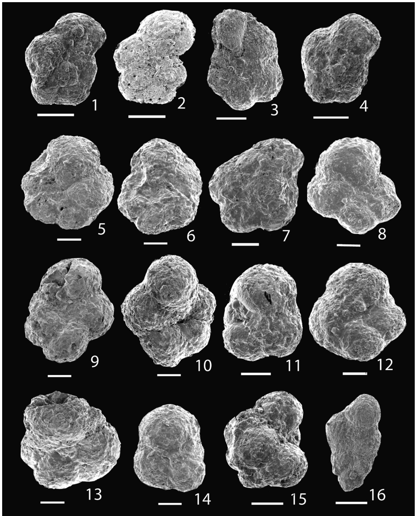
Plate 2. Tiny early Danian species from the lower P. eugubina Zone Pla(1) at Coxquihui, Mexico. All specimens are from the 20 cm thick interval between the 1 cm thin spherule layer 1 and 60 cm thick spherule layer 2. Note that Coxquihui and Beloc have the same tiny early Danian species associated with spherule layers within the early Danian P. eugubina Zone Pla(1). All specimens are from the 38–63 \mu\text{m} size fraction (scale bar = 20 \mu\text{m} ). (1–3) Parvularugoglobigerina longiapertura , (4–8) P. eugubina , (9, 10) Eoglobigerina edita , (11) Eoglobigerina eobulloides , (12–14) Globoconusa daubjergensis , (15) P. extensa (= G. conusa ), (16) Woodringina hornerstownensis .
