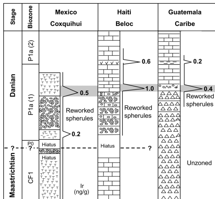
Fig. 7. Correlation of K/T boundary sections at Coxquihui, Haiti (Beloc) and Guatemala (Caribe). Note that at Caribe and Beloc the spherule-rich layers are in the early Danian Zone Pla(1), similar to the upper spherule layer at Coxquihui. All three sections contain small Ir anomalies in the Danian Zone Pla. At Coxquihui, the small Ir anomalies at the K/T boundary and Ir anomaly in Zone Pla are separated by pelagic marls. This suggests that in addition to the K/T boundary impact, a second Ir producing event occurred in Zone Pla.
