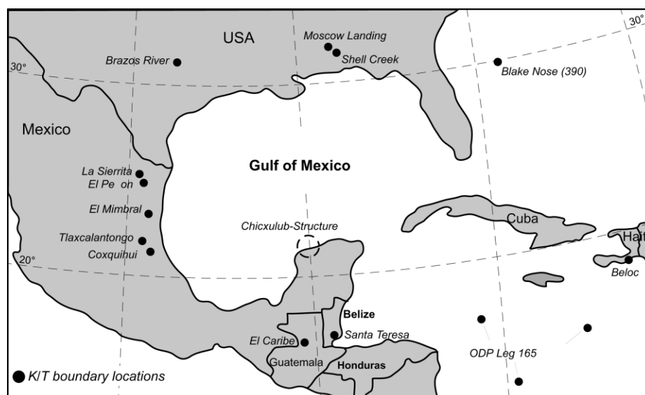
Fig. 1. Location map of K/T boundary sections with spherule-rich deposits (SRDs) around the Gulf of Mexico and the Caribbean.
