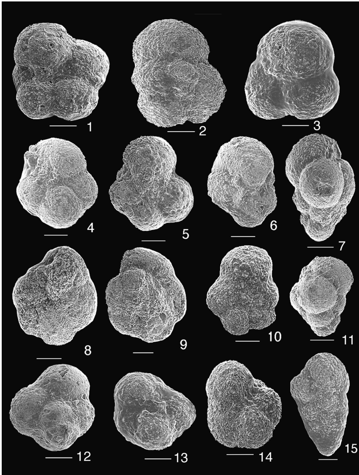
Plate 1. Tiny early Danian species from the lower P. eugubina Zone Pla(1) at Beloc, Haiti. Compare these small species with those shown for the same stratigraphic interval at Coxquihui in Plate 2 . All specimens are within the 38–63 \mu\text{m} size fraction (scale bar = 20 \mu\text{m} ) and were taken from the interval below the Ir and PGE anomalies (for details see Keller et al., 2001 ). (1) Eoglobigerina edita , (2, 3) Eoglobigerina eobulloides , (4, 5) Eoglobigerina fringa , (7, 11) Guembelitra cretacea , (8, 9) Parvularugoglobigerina longiapertura , (10) P. eugubina , (12, 13) P. extensa (= G. conusa ), (14) Globoconusa daubjergensis , (15) Woodringina hornerstownensis .
