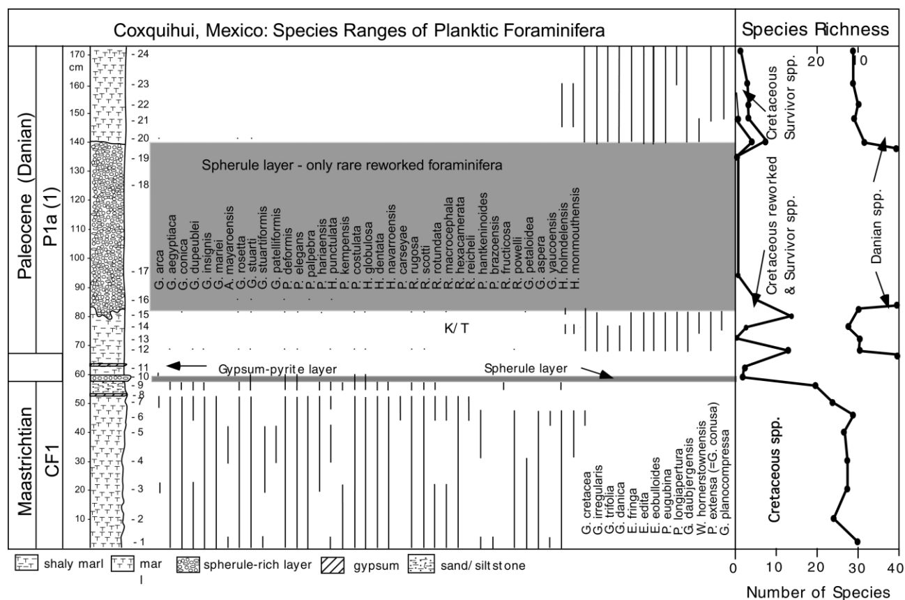
Fig. 5. Planktic foraminiferal species ranges and richness across the K/T boundary at Coxquihui, State of Veracruz, Mexico. Note that the thin spherule layer 1 is located at or close to the K/T boundary. Spherule layer 2 is within the lower part of the P. eugubina Zone, or Pla(l). The early Danian species are very small and can only be recovered in the 38–63 \mu\text{m} size fraction.
