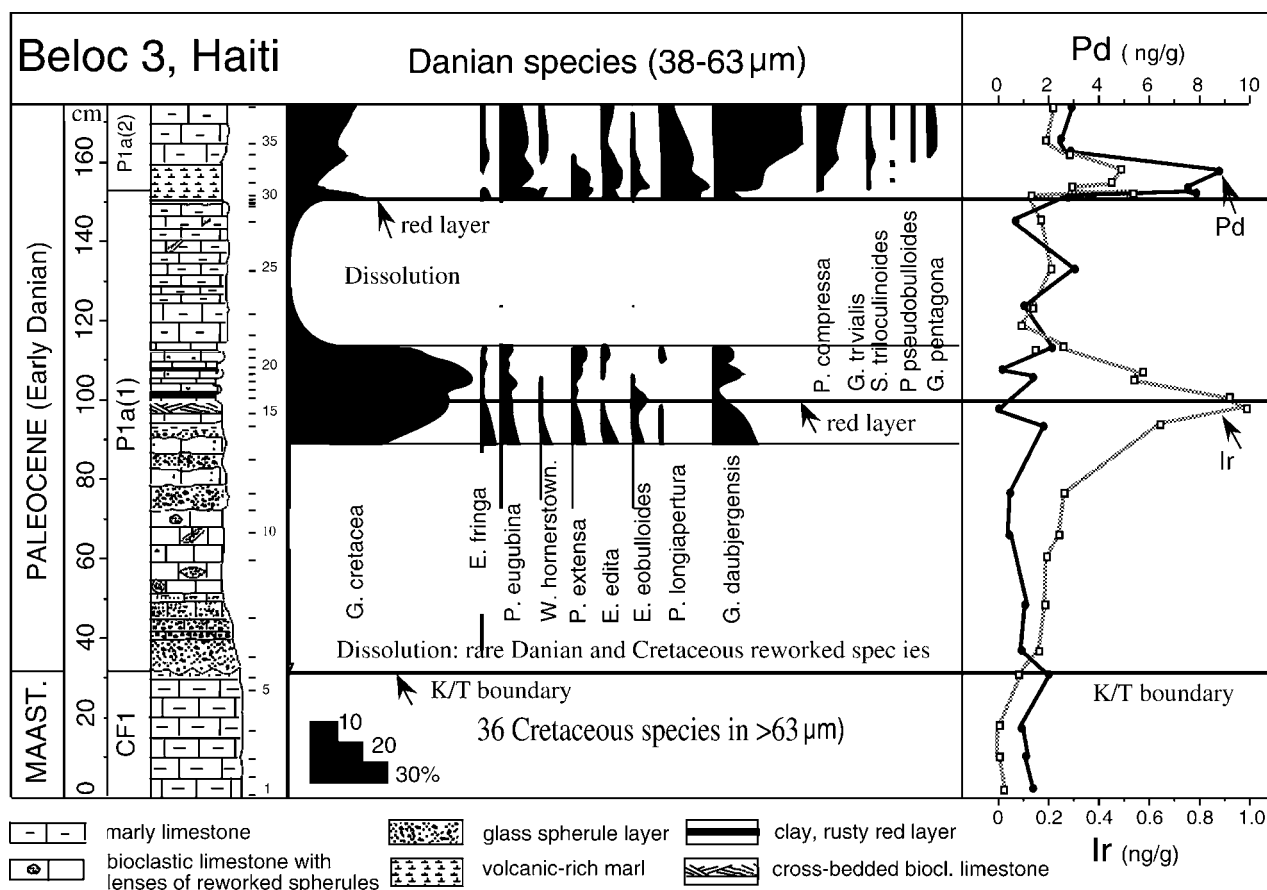
Fig. 2. Spherule deposits, Pd and Ir anomalies and relative abundances of planktic foraminifera in the early Danian at Beloc, Haiti. Note that the first abundant early Danian assemblage and Ir anomaly above the spherule deposit is stratigraphically coeval with that at Coxquihui in Fig. 6.
