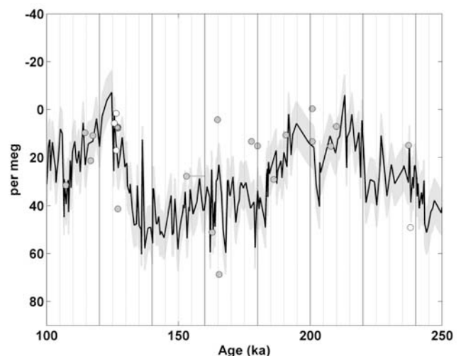
Figure 7. The ^{17}\Delta of O_2 [Blunier et al., 2002; M. Bender et al., unpublished data, 2005] versus time plotted (solid line) with \pm 1\sigma (shaded area). Shaded circles are ^{17}\Delta of O_2 of the disturbed section of the GISP2 core plotted versus best estimate ages. Four open circles are uniquely dated samples.
