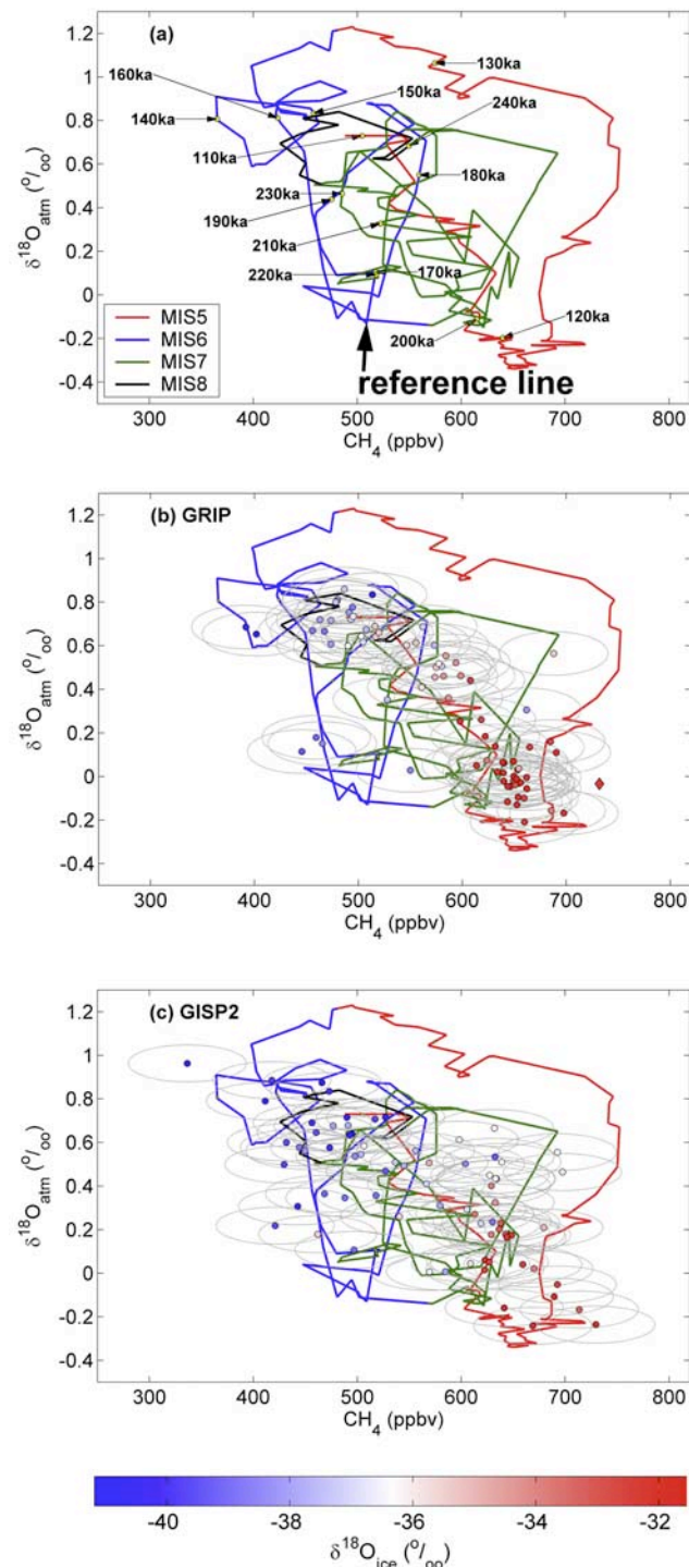
Figure 2. (a) Trajectory of \text{CH}_4 and \delta^{18}\text{O}_{\text{atm}} records derived from the Vostok core between 110 ka and 250 ka on the GT4 timescale, when corrected for the interhemispheric gradient (called “reference line” in the text). Different line colors correspond to different marine isotope stages: red, MIS 5; blue, MIS 6; green, MIS 7; and black, MIS 8. (b) GRIP and (c) GISP2 data from the disturbed section of the core, shown as solid circles colored in shades of red and blue. Color represents \delta^{18}\text{O}_{\text{ice}} at the same sample. Gray ellipses surrounding each data point are uncertainty ranges. A diamond shown in Figure 2b indicates that the sample is not compatible with any age between 250 ka and 101 ka, possibly because of its high methane concentration. Note that we define MIS 5 as starting at 133 ka, MIS 6 at 198 ka, and MIS 7 at 240 ka on the basis of a the Vostok plot of \delta\text{D}_{\text{ice}} versus time (GT4 timescale).
