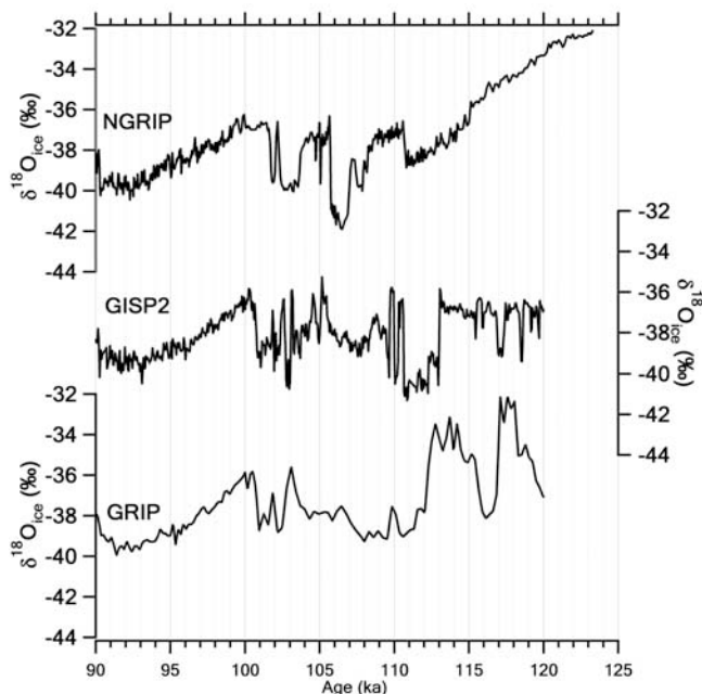
Figure 1. Comparison of \delta^{18}\text{O}_{\text{ice}} of GISP2 [Grootes et al., 1993], GRIP [Dansgaard et al., 1993] and NGRIP [North Greenland Ice Core Project Members, 2004] ice cores between 125 ka and 90 ka. GISP2, GRIP and NGRIP curves are plotted on the GISP2 timescale [Meese et al., 1994; Sowers et al., 1993] until 101 ka. This chronology is extrapolated for a period prior to 101 ka as if there had been no basal mixing in GISP2 and GRIP. NGRIP chronology prior to 101 ka is from Landais et al. [2006].
