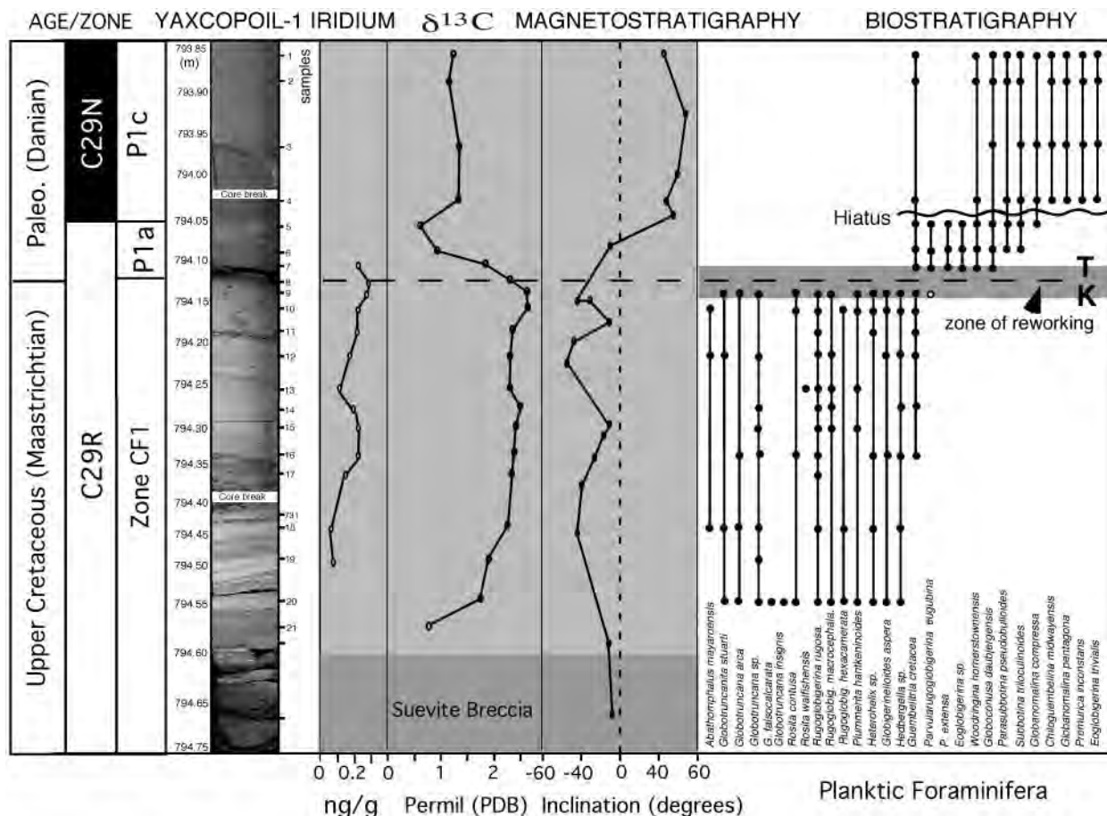
Fig. 2. Five sediment and age-related proxies reveal Late Maastrichtian pelagic sediments overlying the impact breccia in the Chicxulub core Yax-1. Note that zones P0, most of P1a, and probably the uppermost part of zone CF1 are missing. In addition, the hiatus at 794.05 m marks the loss of zone P1b and the lower part of P1c. The absence of the Ir anomaly is likely due to the hiatus that spans the K-T boundary.
