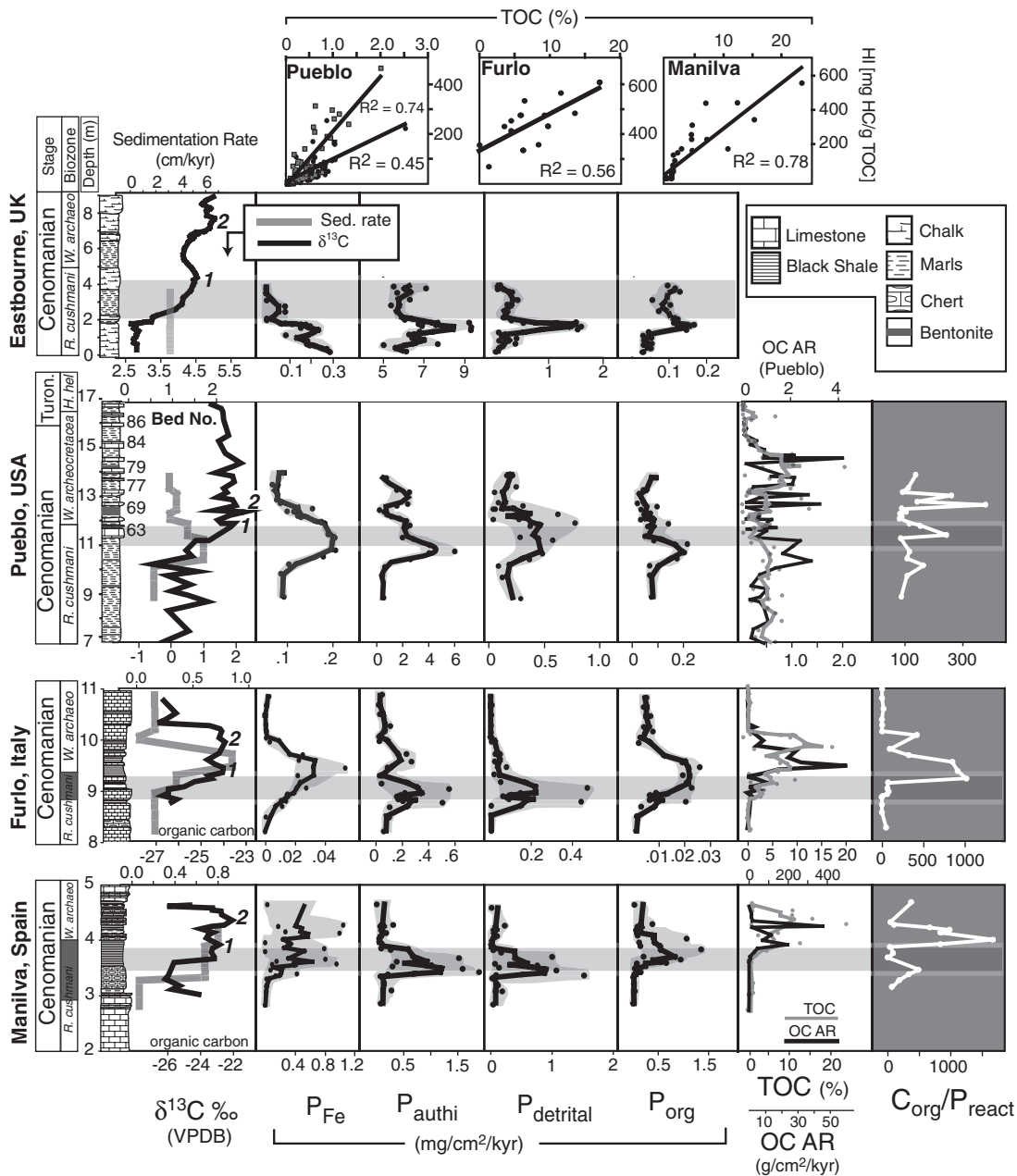
Figure 2. Phosphorus (P) speciation with accumulation rates (mg/cm 2 /k.y.) in four sections, plotted against corresponding δ 13 C curves. Gray shaded area highlights interval in time between peak in P mass accumulation rates and first peak in δ 13 C values. Percentages for total organic carbon, hydrogen indices, and C org /P reactive molar ratios are also shown. Smoothed lines are 3-point moving averages. Scatter plots are correlations between total organic carbon (TOC) and hydrogen indices. Two correlations are made for Pueblo (black circles and gray squares represent terrestrial and/or oxidized and marine organic matter, respectively). Rotalipora cushmani biozones in Furlo and Manilva are extended with gray bars, which represent probable extinction level. All P speciation data can be found in Appendix 1 (also see Appendix 2 for more details; see footnote 1). Tur.—Turonian; OC AR—organic carbon accumulation rate; VPDB—Vienna Peedee belemnite.
